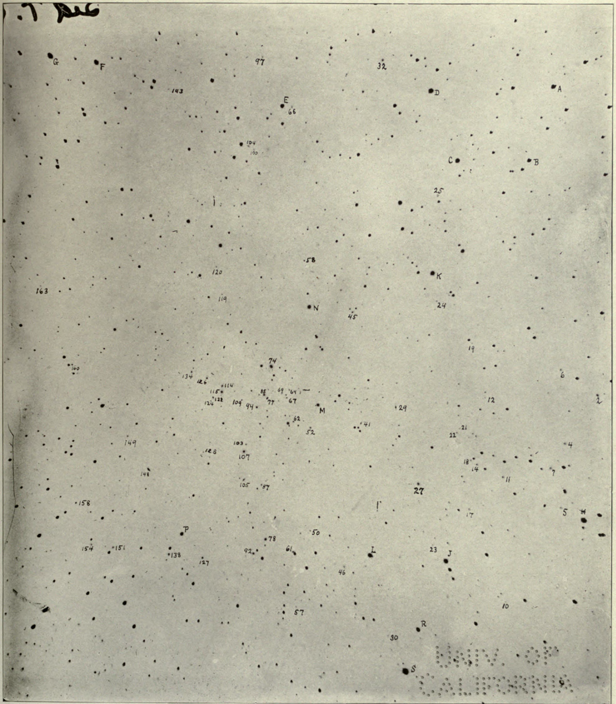
ENLARGED NEGATIVE OF FIELD III Center at \alpha=11^{\text{h}}4^{\text{m}} , \delta=+29^{\circ}30' For identification of lettered stars see page 73
